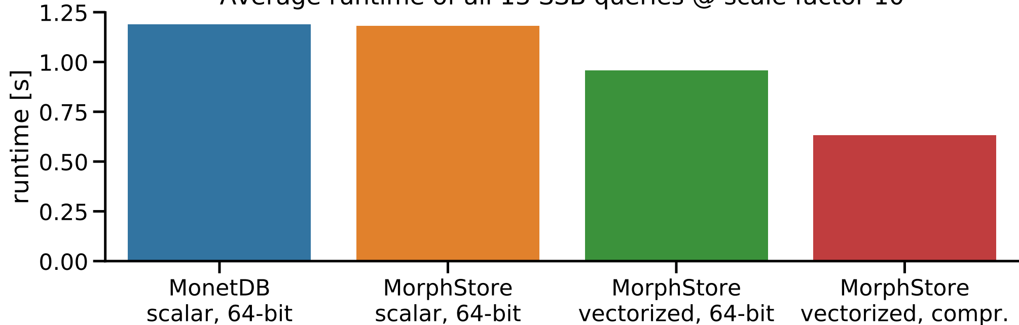
Average runtime of all 13 SSB queries @ scale factor 10
